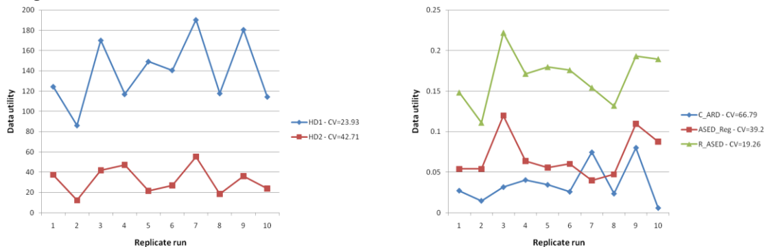
Figure 1 –Utility measures over 10 replicates for the scenario based on the balanced method with a swapping rate of 3%, five swapping variables, 384 possible swapping cells and 8,153 observations
